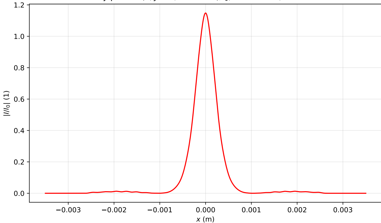
Intensity profile I(x, y = 0, z = 1.433)/I_0 , P_{in}=1.0P_{cr} , artificial time
